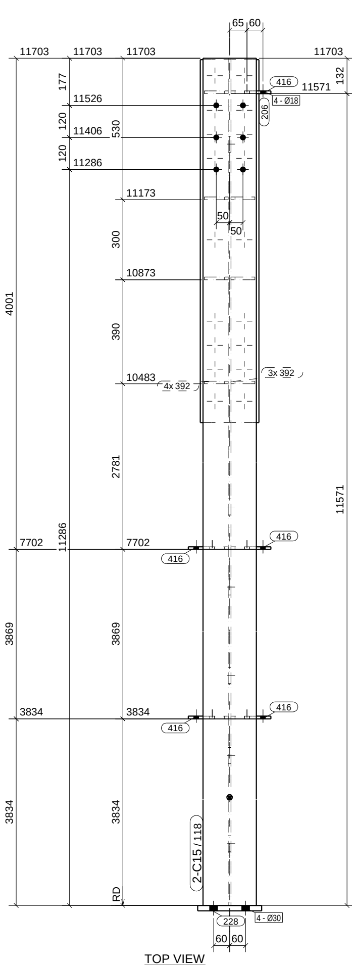
TOP VIEW
